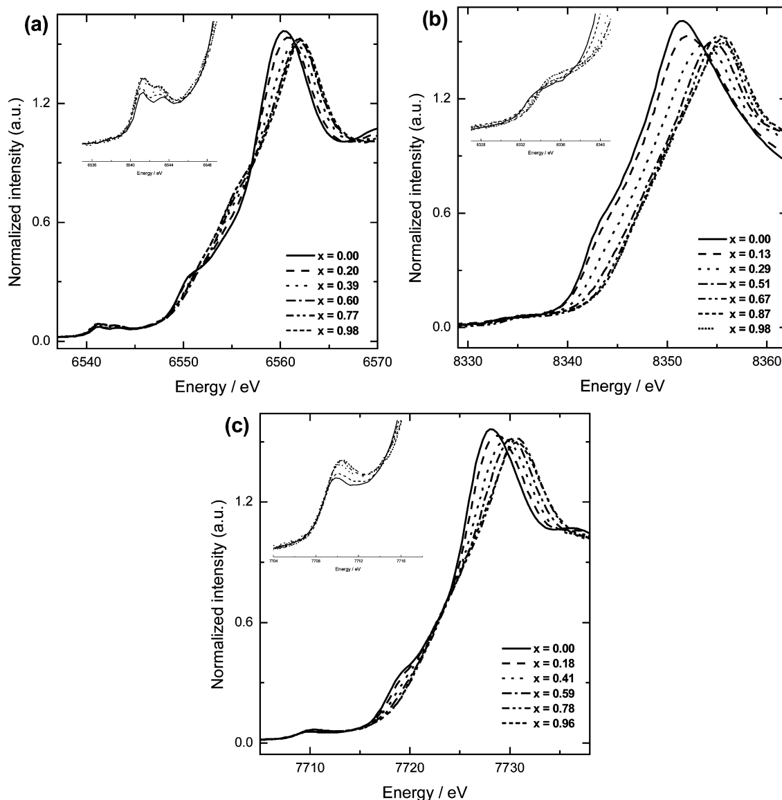
Figure 3. Normalized (a) Mn, (b) Ni, and (c) Co K-edge XANES spectra of \text{Li}_{1-x}\text{Co}_{1/3}\text{Ni}_{1/3}\text{Mn}_{1/3}\text{O}_2 electrode during charge.
