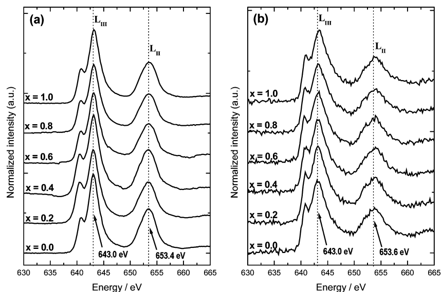
Figure 5. Normalized Mn L_{II,III} -edge XAS spectra of \text{Li}_{1-x}\text{Co}_{1/3}\text{Ni}_{1/3}\text{Mn}_{1/3}\text{O}_2 electrode at different x values using (a) PEY method and (b) FY method.
