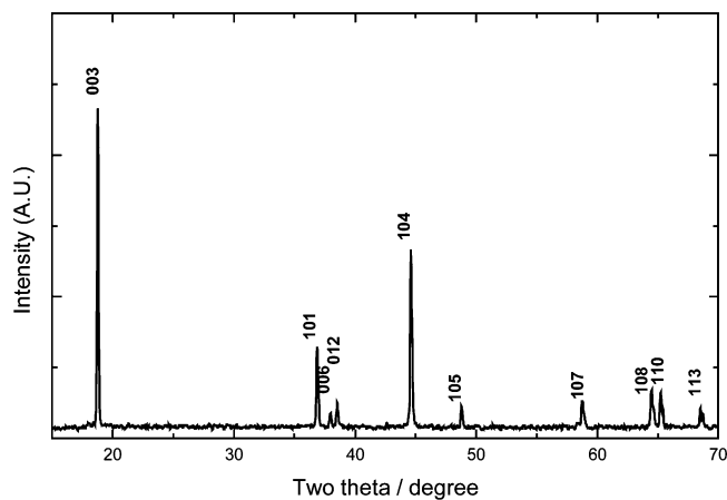
Figure 1. XRD pattern of \text{LiCo}_{1/3}\text{Ni}_{1/3}\text{Mn}_{1/3}\text{O}_2 powders synthesized at 900 °C.
